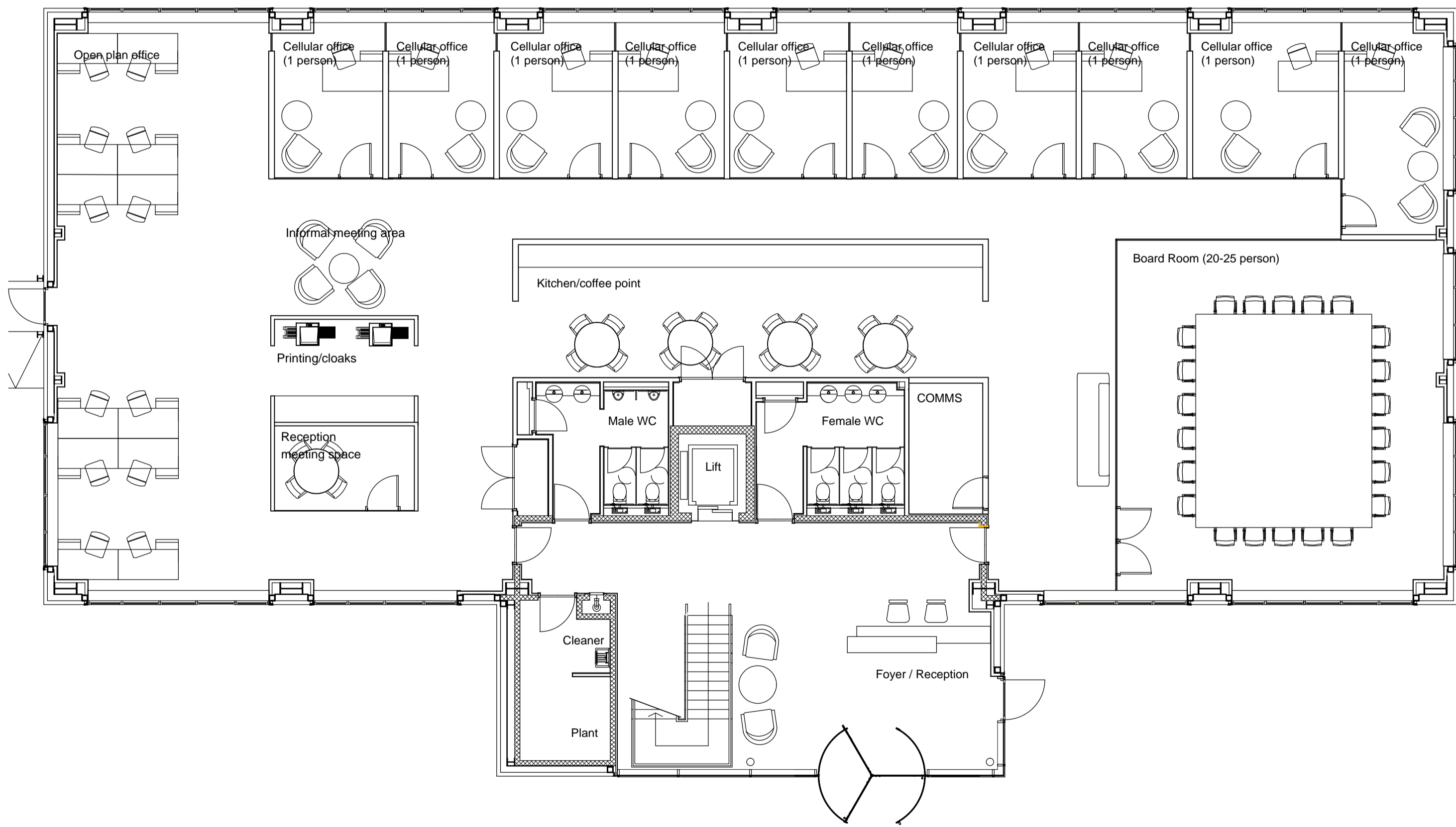
GROUND FLOOR
