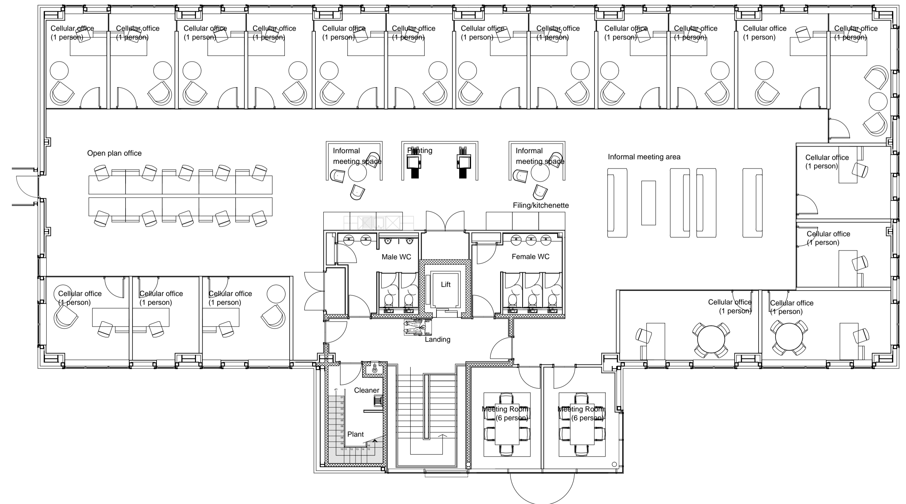
SECOND FLOOR
